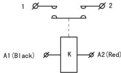
K Two Jiont Magnetic Retention (Two Jiont Self-locking)
