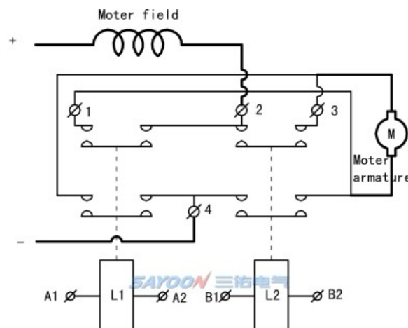
Paired Double Pole Single Throw Contactor for motor reversing. 1.2.3.4 Contact Terminal A1. A2. B1. B2 for the two sets of coil terminal
